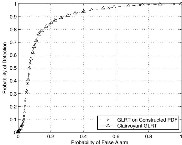
Figure 2: ROC curves for the GLRT using the constructed PDF and the clairvoyant GLRT with uncorrelated Gaussian mixture noise.
